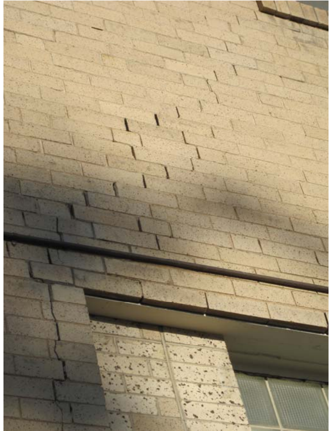
LEL9340 IN-PLANE CORBEL PATTERN CRACKING ABOVE NORTH END OF FOURTH WINDOW FROM THE NORTH ON THE WEST ELEVATION
