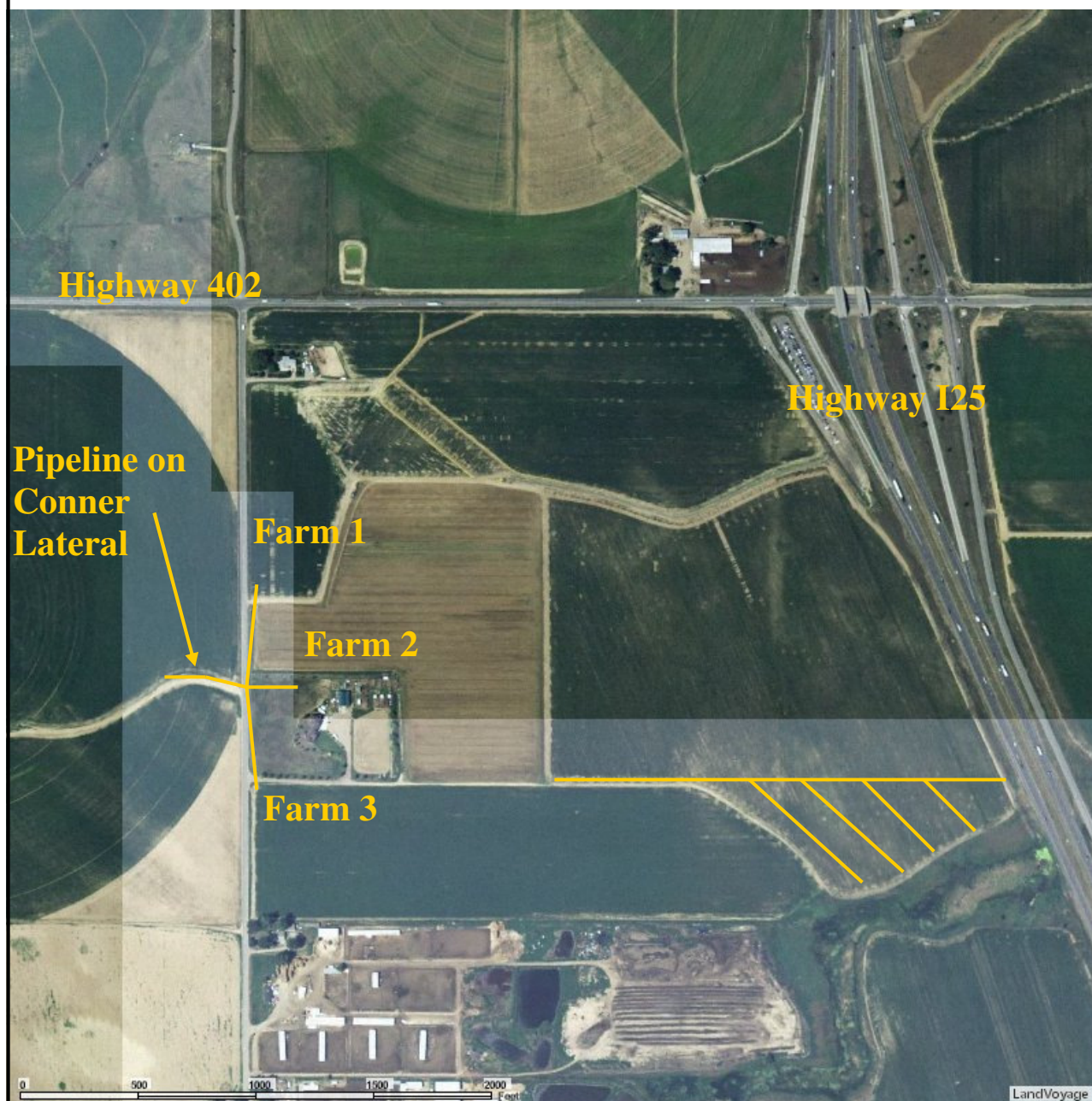
Irrigation Pipeline to City of Loveland Farm, I25 and Highway 402
